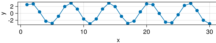
Figure 3.5: Sine function.
