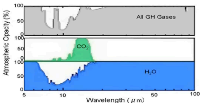
Figure 2: Greenhouse Heat Trapping Capacity.
